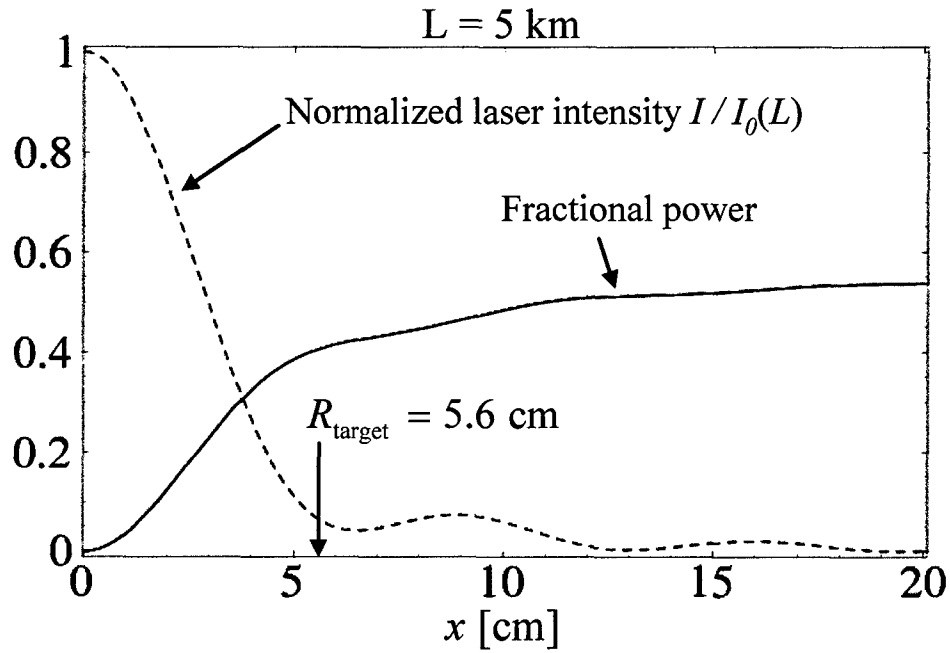
Figure 3: Fractional power (solid curve) and normalized laser intensity (dashed curve) versus transverse coordinate x at a range of L = 5 \text{ km} for the coherent beam director of Fig. 2. Fractional power is defined as the power contained within a circle of radius x normalized to the total transmitted power. The radius of a circular target with an area of 100 \text{ cm}^2 is R_{\text{target}} = 5.6 \text{ cm} . Laser intensity is normalized to I_0(L) = 2.8 \text{ kW/cm}^2 , which denotes the on-axis laser intensity at z = L . The power on target is 100 \text{ kW} .
