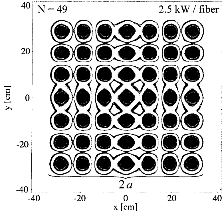
Figure 6: Fiber array for incoherent beam combining. Figure shows laser intensity profile at the beam director ( z = 0 ) for 49 fibers arranged in a square array. The Gaussian spot size of each laser is 4 cm. The individual lasers are separated by 9.6 cm. The size of the array is a = 33 cm and the power per fiber is taken to be P_{\text{fiber}} = 2.5 kW. The total transmitted power is 123 kW. The power on target is 100 kW for a target with a circular area of A_{\text{target}} = 100 \text{ cm}^2 at a range of L = 5 km.
