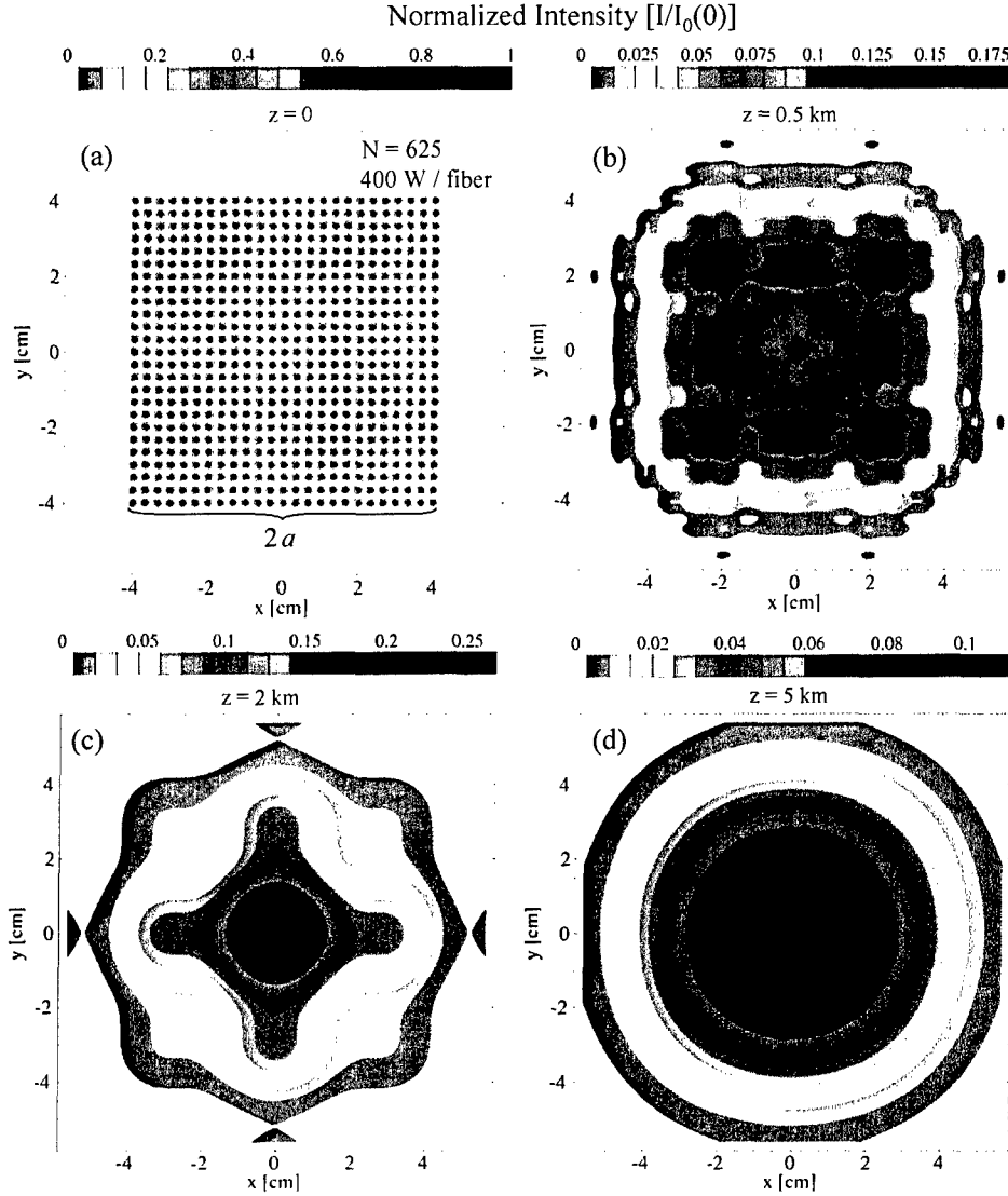
Figure 2: A fiber array for coherent beam combining. (a) Laser intensity profile at the beam director for 625 fibers. x and y denote transverse coordinates. Intensity is normalized to I_0(0) , which denotes the on-axis intensity at z = 0 . The Gaussian spot size of each laser is 1 mm. The individual lasers are separated by 2R_c = 3.3 \text{ mm} . The size of the array is a = 4 \text{ cm} and the power per fiber is assumed to be P_{\text{fiber}} = 400 \text{ W} . The total transmitted power is 250 kW. Figures (b), (c), and (d) show the intensity profile at z = 0.5 \text{ km} , 2 \text{ km} , and 5 \text{ km} , respectively. The power on target is 100 kW for a target with a circular area of A_{\text{target}} = 100 \text{ cm}^2 at a range of L = 5 \text{ km} .
