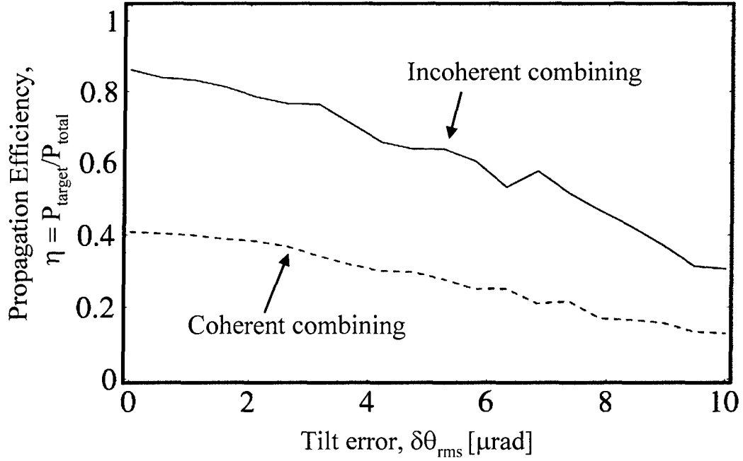
Figure 8: Propagation efficiency, \eta = P_{\text{target}} / P_{\text{total}} versus rms tilt error, \delta\theta_{rms} , for the coherent (dashed curve) and incoherent (solid curve) beam combining examples of Figs. 2 and 6. Propagation efficiency is defined as the ratio of the power on target to the transmitted power. The target is taken to have a circular area of A_{\text{target}} = 100 \text{ cm}^2 at a range of L = 5 \text{ km} . Each laser is given a random tilt error relative to the propagation axis with rms value \delta\theta_{rms} .
