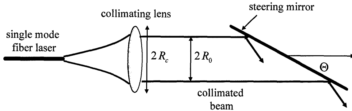
Figure 5: An expanded diagram of a single fiber laser system used in the incoherent beam combining configuration of Fig. 4. The individual lasers are Gaussian ( \text{TEM}_{00} ) modes. The laser from the fiber diffracts to a spot size R_0 \sim 4 \text{ cm} and passes through a collimating lens of radius R_c = 1.2 R_0 . A steering mirror directs the beam to the target. The steering mirror angle \Theta is defined with respect to the propagation axis and may have a tilt error denoted by the rms value \delta\theta_{rms} \ll 1 .
