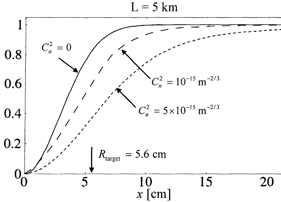
Figure 10: Fractional power versus transverse coordinate x at a range of L = 5 km for the incoherent beam director of Fig. 6. Fractional power is defined as the power contained within a circle of radius x normalized to the total transmitted power. The radius of a circular target with an area of 100 \text{ cm}^2 is R_{\text{target}} = 5.6 \text{ cm} . Curves represent cases with no atmospheric turbulence, weak turbulence ( C_n^2 = 10^{-15} \text{ m}^{-2/3} ), and moderate turbulence ( C_n^2 = 5 \times 10^{-15} \text{ m}^{-2/3} ).
