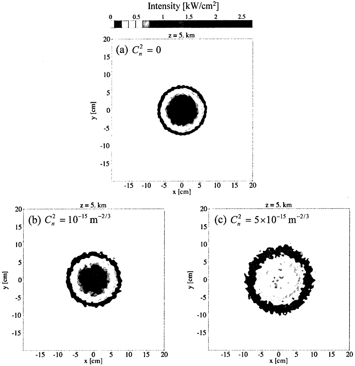
Figure 9: Average intensity at the target plane ( L = 5 km) for cases of (a) no atmospheric turbulence, (b) weak turbulence ( C_n^2 = 10^{-15} \text{ m}^{-2/3} ), and (c) moderate turbulence ( C_n^2 = 5 \times 10^{-15} \text{ m}^{-2/3} ) for the incoherent combining example of Fig. 6.
