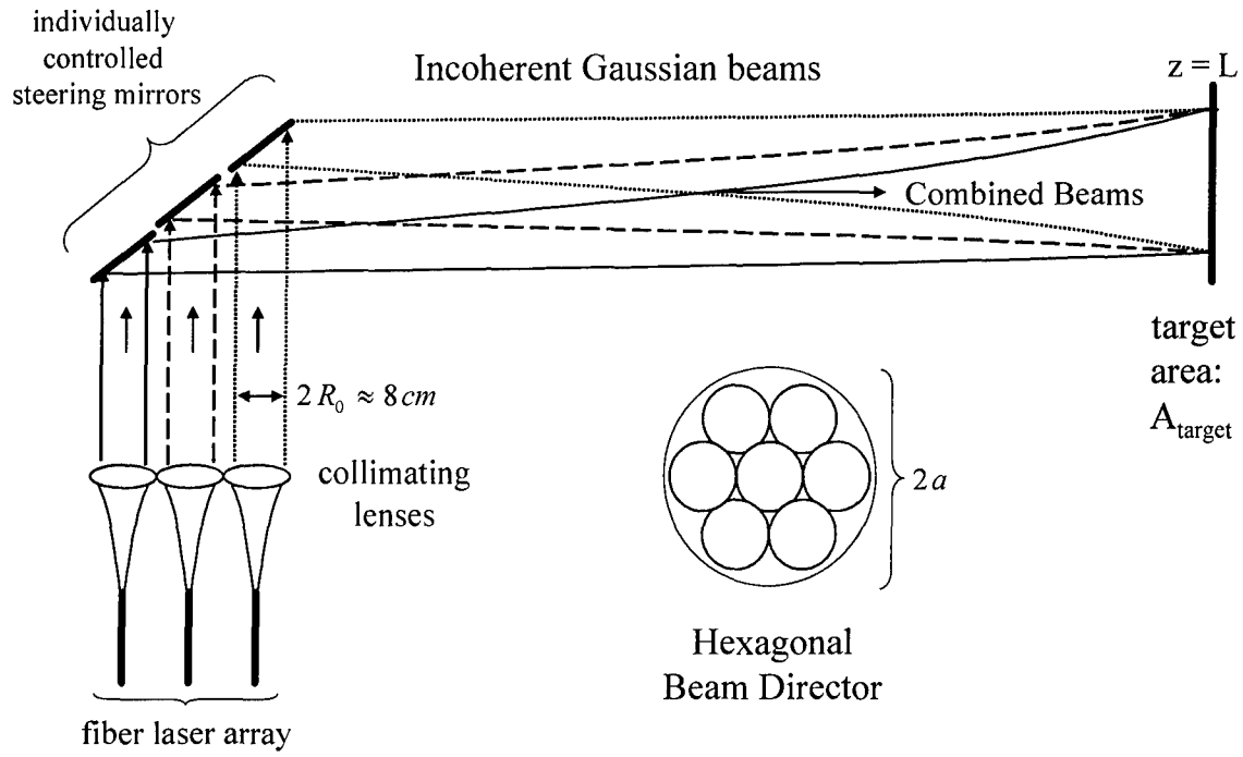
Figure 4: Schematic of incoherent beam combining configuration. The individual lasers are Gaussian ( TEM_{00} ) modes. From the fiber, each laser diffracts to a spot size R_0 \sim 4 \text{ cm} and passes through a collimating lens of radius R_c = 1.2 R_0 . Individually controlled steering mirrors direct each beam to the target. To minimize diffractive spreading, the range to the target must be < 2 Z_R , where Z_R = \pi R_0^2 / \lambda = 5 \text{ km} is the Rayleigh length associated with the individual beams. The total transmitted power is N P_{\text{fiber}} and the beam director array dimension is a \sim \sqrt{N} R_c . An example of a hexagonal array of seven fibers is also shown.
