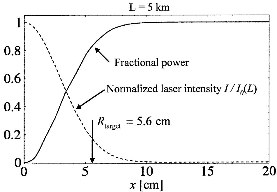
Figure 7: Fractional power (solid curve) and normalized laser intensity (dashed curve) versus transverse coordinate x at a range of L = 5 \text{ km} for the incoherent beam director of Fig. 6. Fractional power is defined as the power contained within a circle of radius x normalized to the total transmitted power. The radius of a circular target with an area of 100 \text{ cm}^2 is R_{\text{target}} = 5.6 \text{ cm} . Laser intensity is normalized to I_0(L) = 2.2 \text{ kW/cm}^2 , which denotes the on-axis laser intensity at z = L . The power on target is 100 \text{ kW} .
